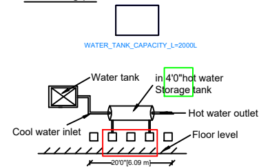
Solar hot water system detailes
