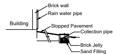
Details of Rain Water Harvesting pit
