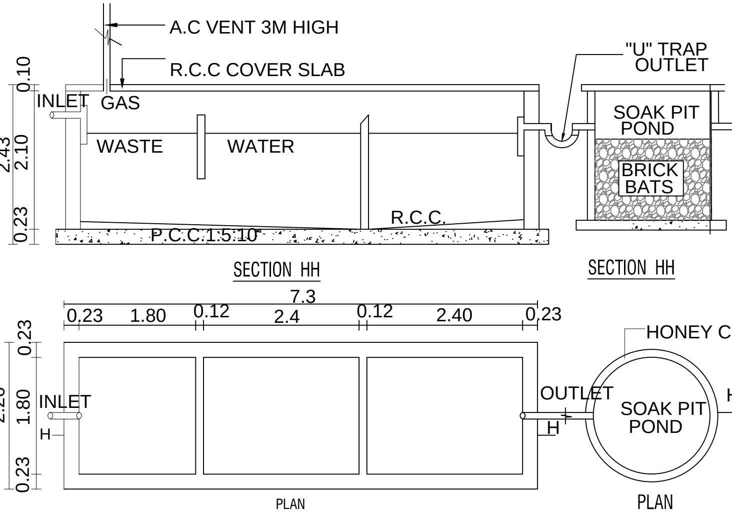
SEPTIC TANK DETAILS (NTS)
