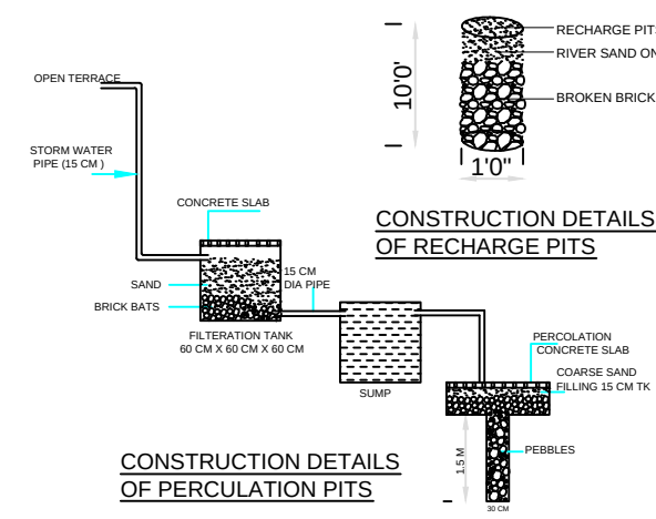
CONSTRUCTION DETAILS OF PERCUSSION PITS
