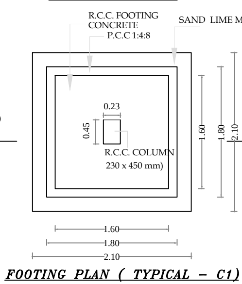
FOUNDATION DETAILS
