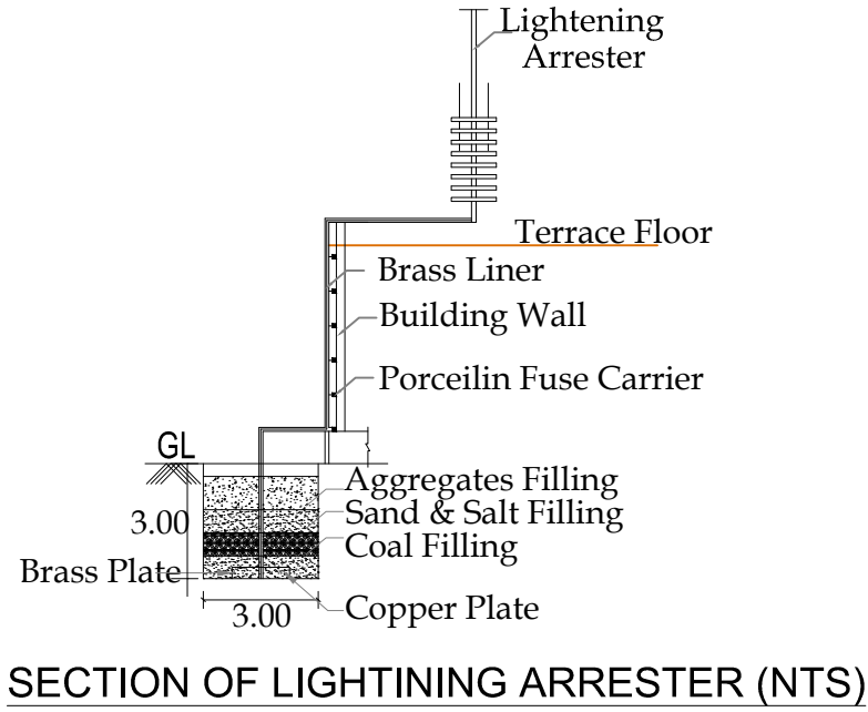
SECTION OF LIGHTNING ARRESTER (NTS)
