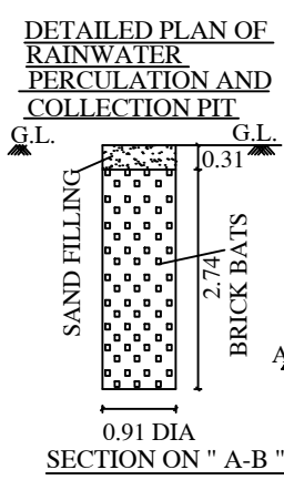
SECTION ON "A-B"
