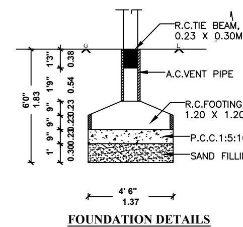
FOUNDATION DETAILS
