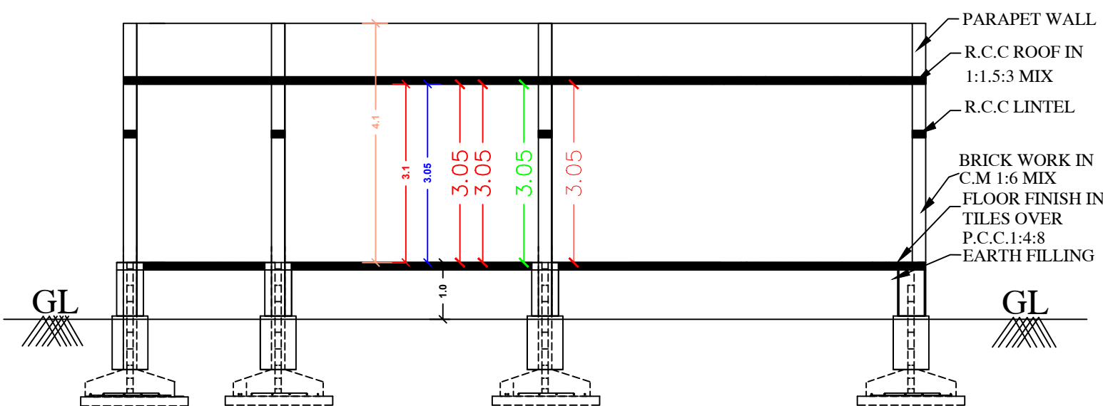
SECTION AA
