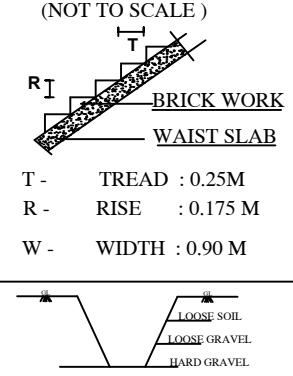
STAIRCASE DETAILS
