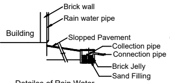
Details of Rain Water Harvesting pit
