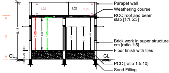
Section "AB"
