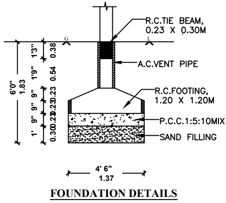
FOUNDATION DETAILS
