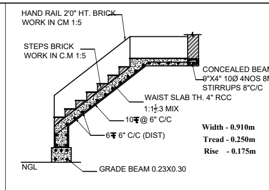
STAIRCASE DETAILS
