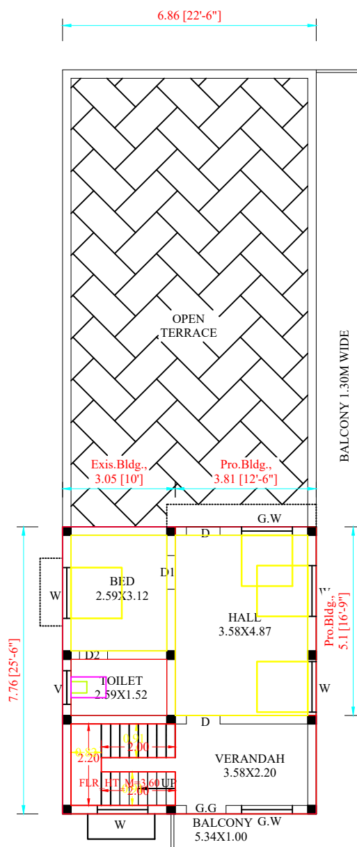
PRO.ADDLSECOND FLOOR PLAN
