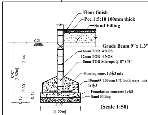
FOUNDATION DETAILS
