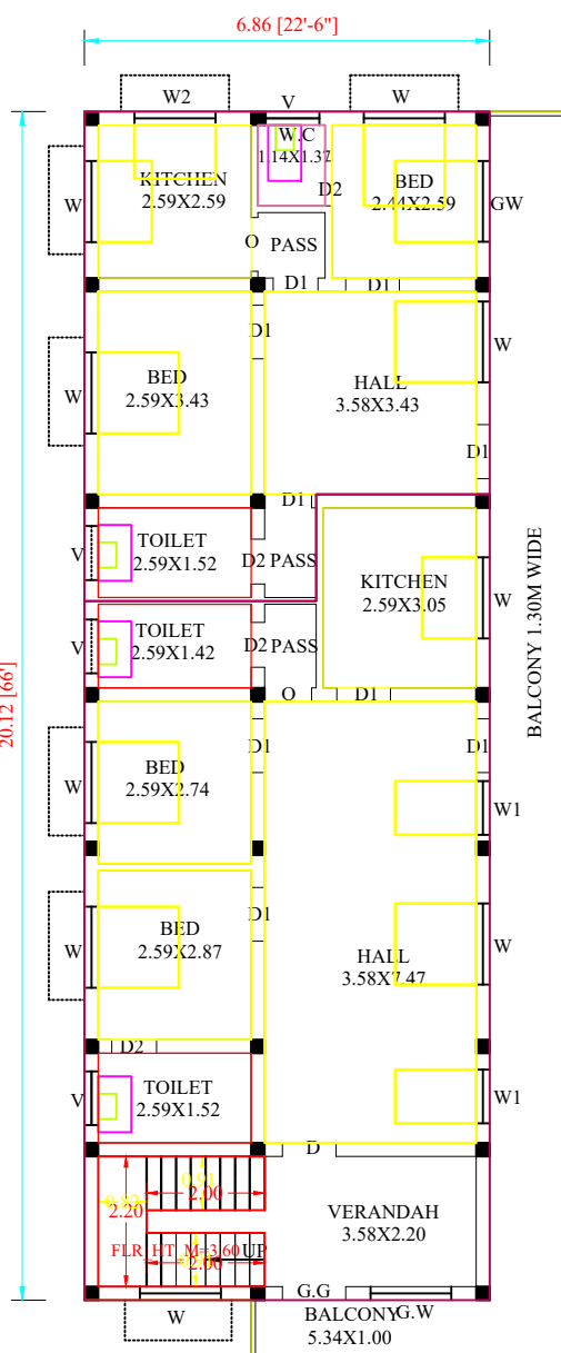
EXIS.FIRST FLOOR PLAN
