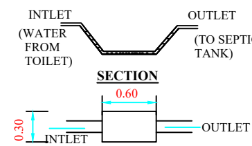
PLAN OF "U" TRAP (Not to Scale)
