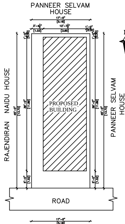
SITE PLAN
