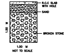
RAIN WATER HARVEST COLLECTION PIT.
