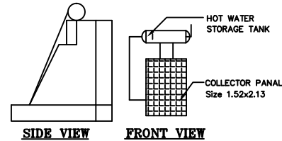
SIDE VIEW FRONT VIEW SOLAR WATER HEATER DETAILS
