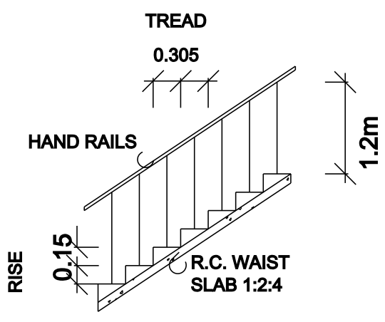
STAIRCASE DETAILS
