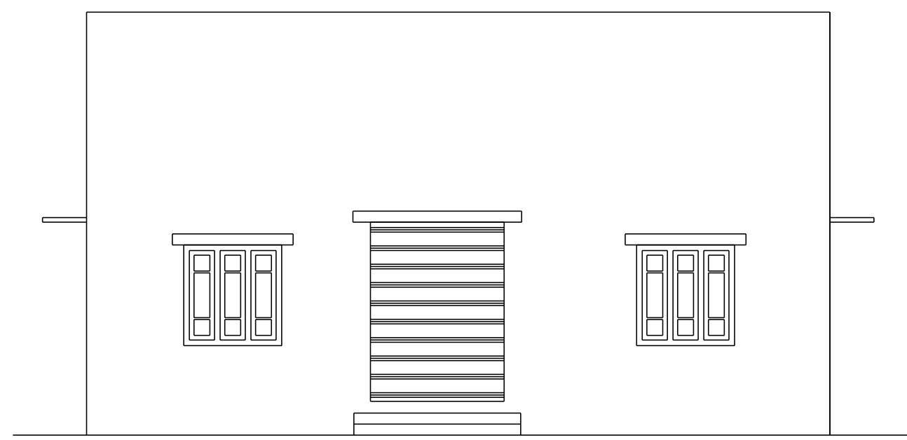
FRONT ELEVATION
