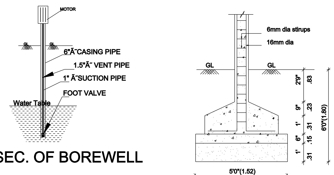
COLUMN FOUNDATION DETAIL
