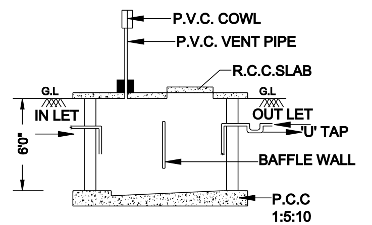
SEC. OF SEPTIC TANK
