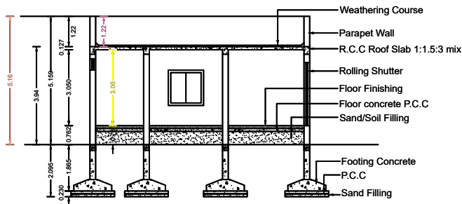
SECTION "A-B"
