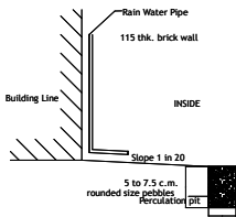
PERCOLATION PIT
