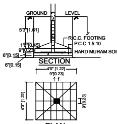
FOUNDATION DETAILS
