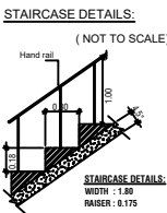
STAIRCASE DETAILS: (NOT TO SCALE)
