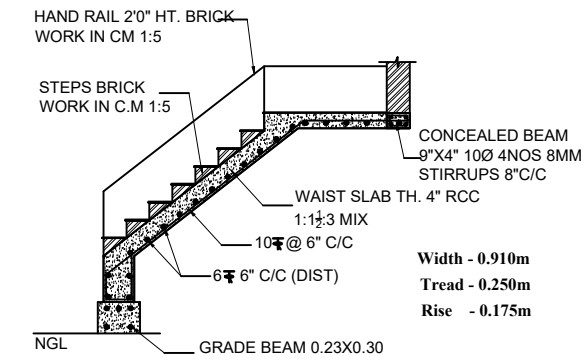
STAIRCASE DETAILS
