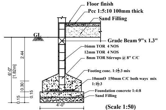
FOUNDATION DETAILS
