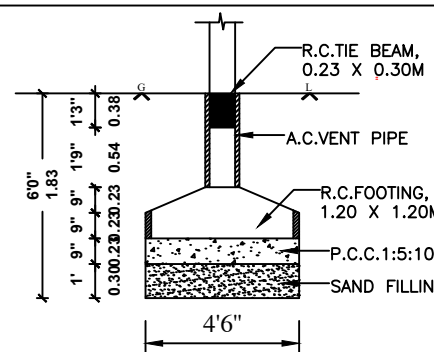
FOUNDATION DETAILS
