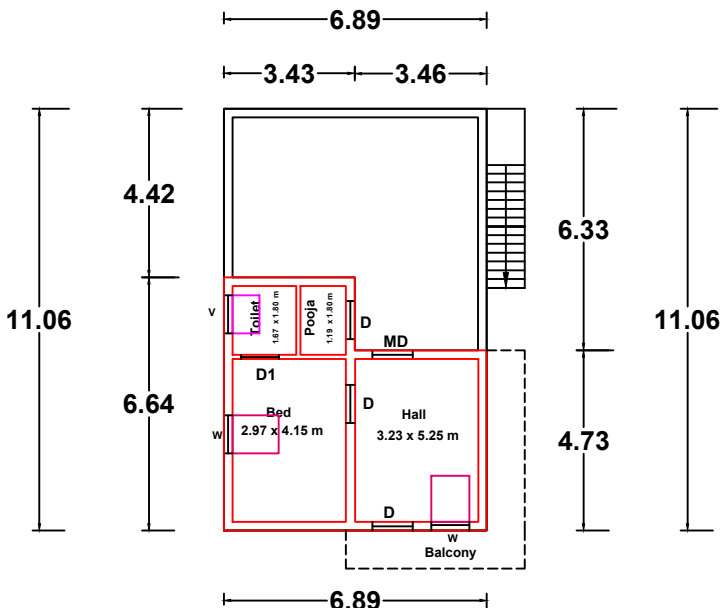
FIRST FLOOR PLAN & OPEN TERRACE
