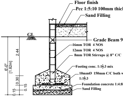
FOUNDATION DETAILS
