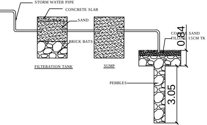
CONSTRUCTION DETAILS OF RECHARGE TRENCH
