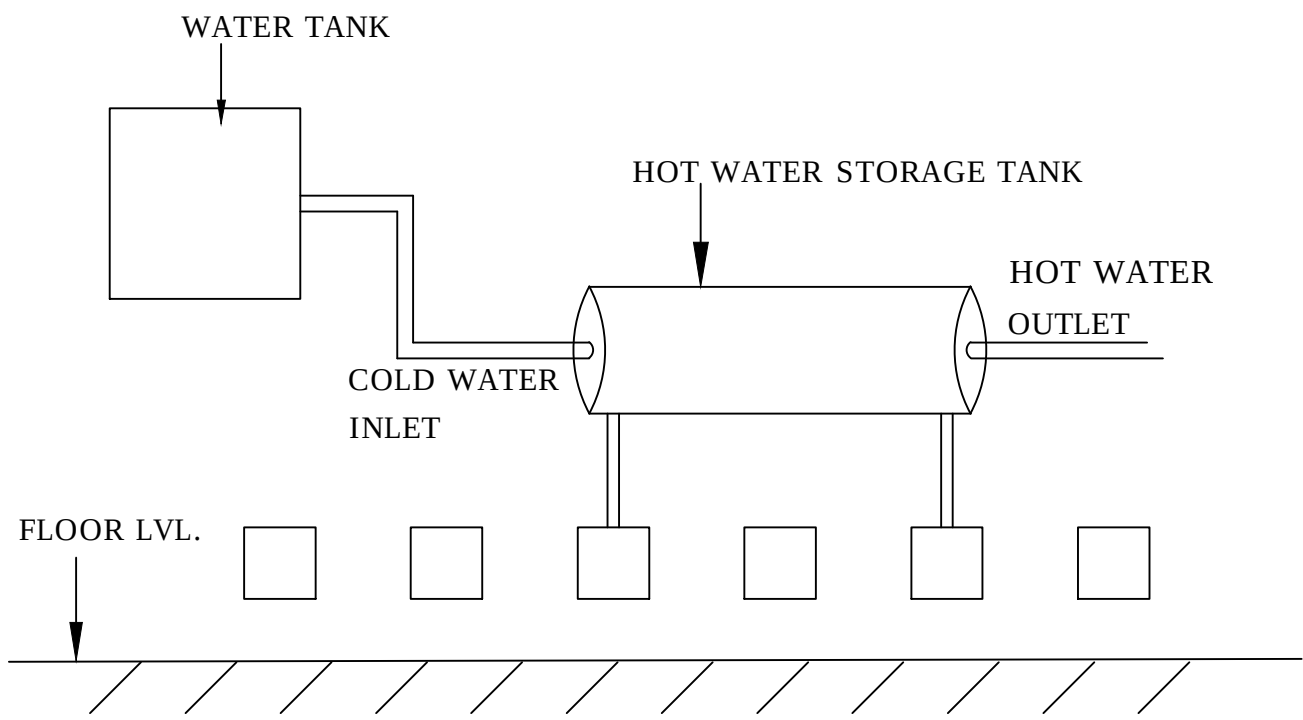
SOLAR WATER HEATER SYSTEM
