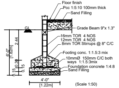
FOUNDATION DETAILS
