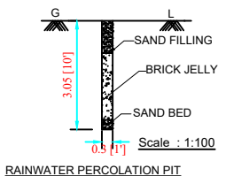
RAINWATER PERCOLATION PIT
