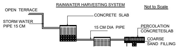
RAINWATER HARVESTING SYSTEM
