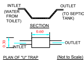
PLAN OF "U" TRAP (Not to Scale)
