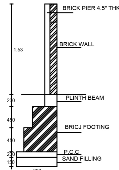
COMPOUND WALL DETAILS NOT TO SCALE
