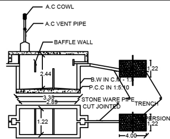
SEPTIC TANK DETAILS NOT TO SCALE
