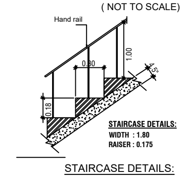
STAIRCASE DETAILS:
