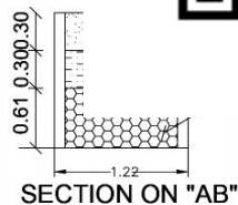
"RAINWATER TANK DETAILS"
