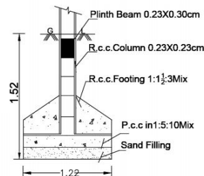
"FOUNDATION DETAILS"
