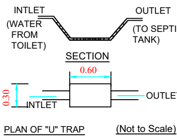
PLAN OF "U" TRAP (Not to Scale)
