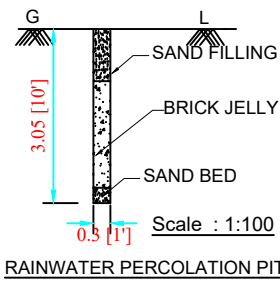
RAINWATER PERCOLATION PIT
