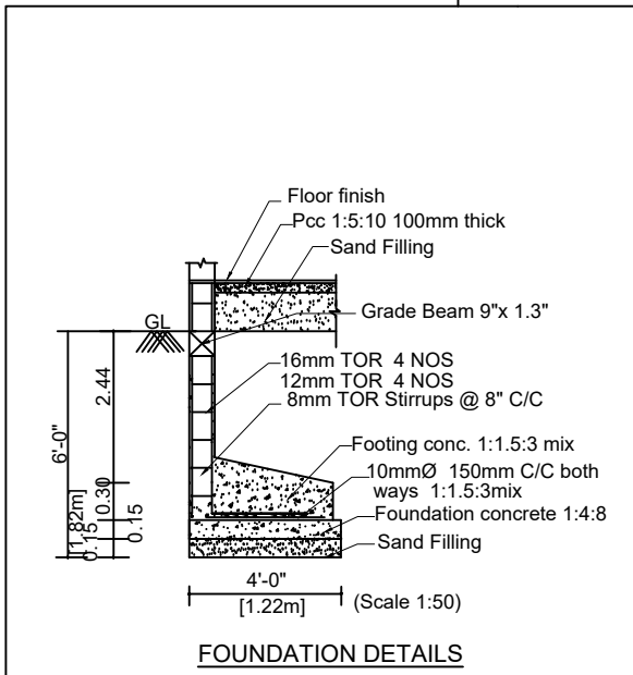
FOUNDATION DETAILS
