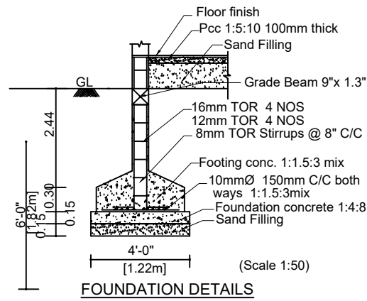
FOUNDATION DETAILS
