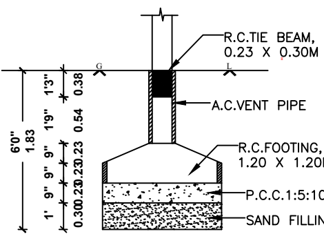
FOUNDATION DETAILS
