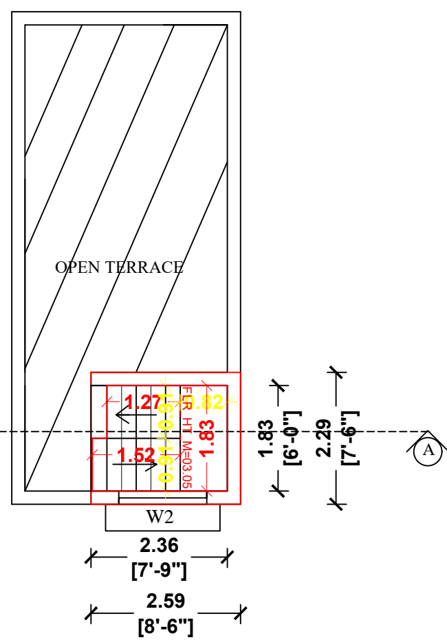
PROPOSED FIRST FLOOR PLAN (HEAD ROOM)
