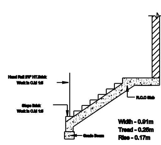
STAIR CASE DETAILS (Scale > 1:100)
