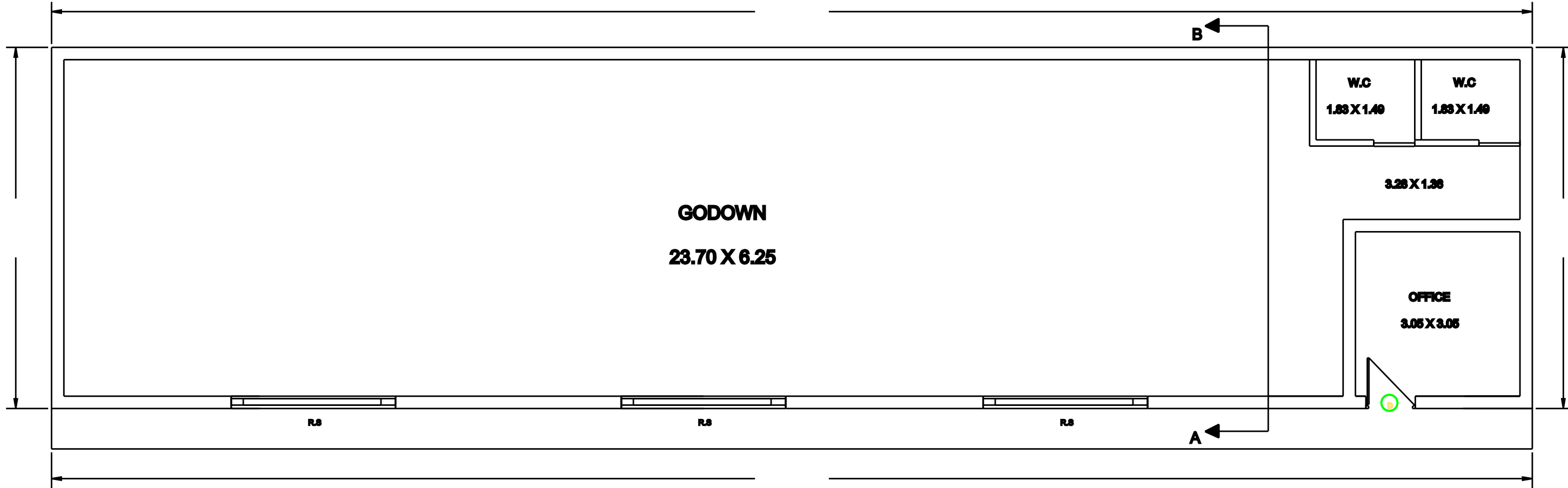
PRO - GROUND FLOOR PLAN
