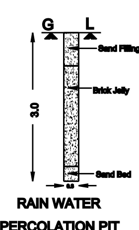
RAIN WATER PERCOLATION PIT (Scale > 1:100)
