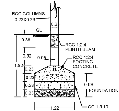
FOUNDATION DETAILS
