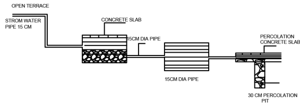
RAIN WATER HARVESTING SYSTEM
