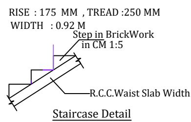
Staircase Detail
