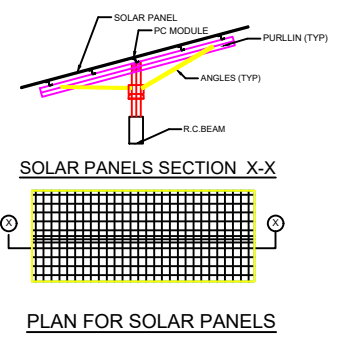
PLAN FOR SOLAR PANELS
