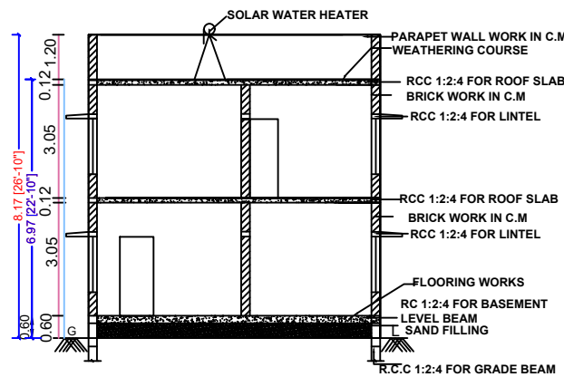
SECTION ON-AA
