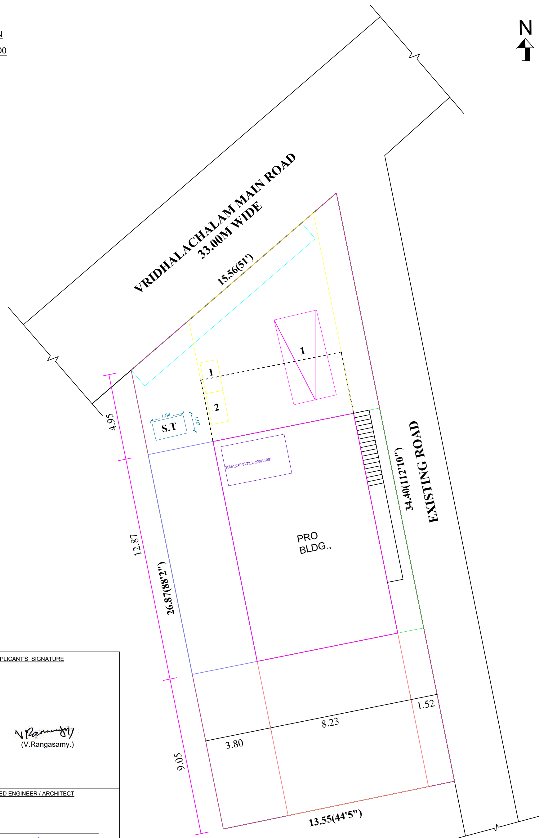
SITE PLAN
