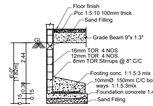
FOUNDATION DETAILS
