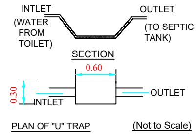
PLAN OF "U" TRAP (Not to Scale)
