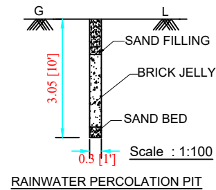
RAINWATER PERCOLATION PIT
