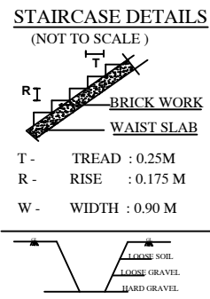
STAIRCASE DETAILS (NOT TO SCALE)
