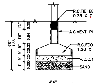
FOUNDATION DETAILS
