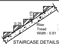
STAIRCASE DETAILS
