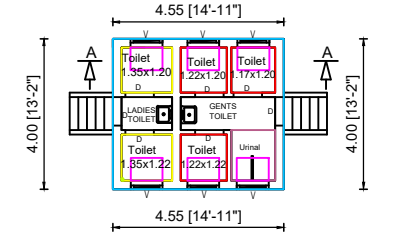
GROUND FLOOR PLAN- (EAST FACE) TOILET- BLOCK 2
