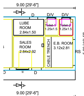
GROUND FLOOR PLAN- (EAST FACE) OFFICE-BLOCK 1
