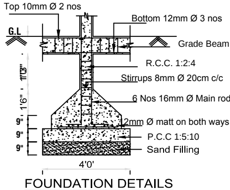
FOUNDATION DETAILS
