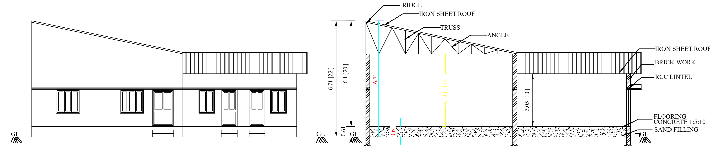
SECTION ON X-X'
