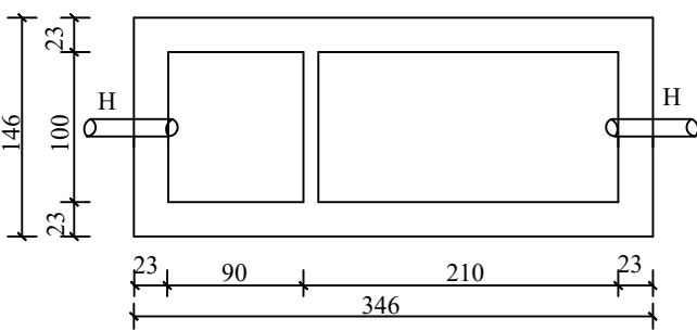
PLAN SEPTIC TANK DETAILS
