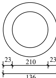
PLAN SOAK PIT
