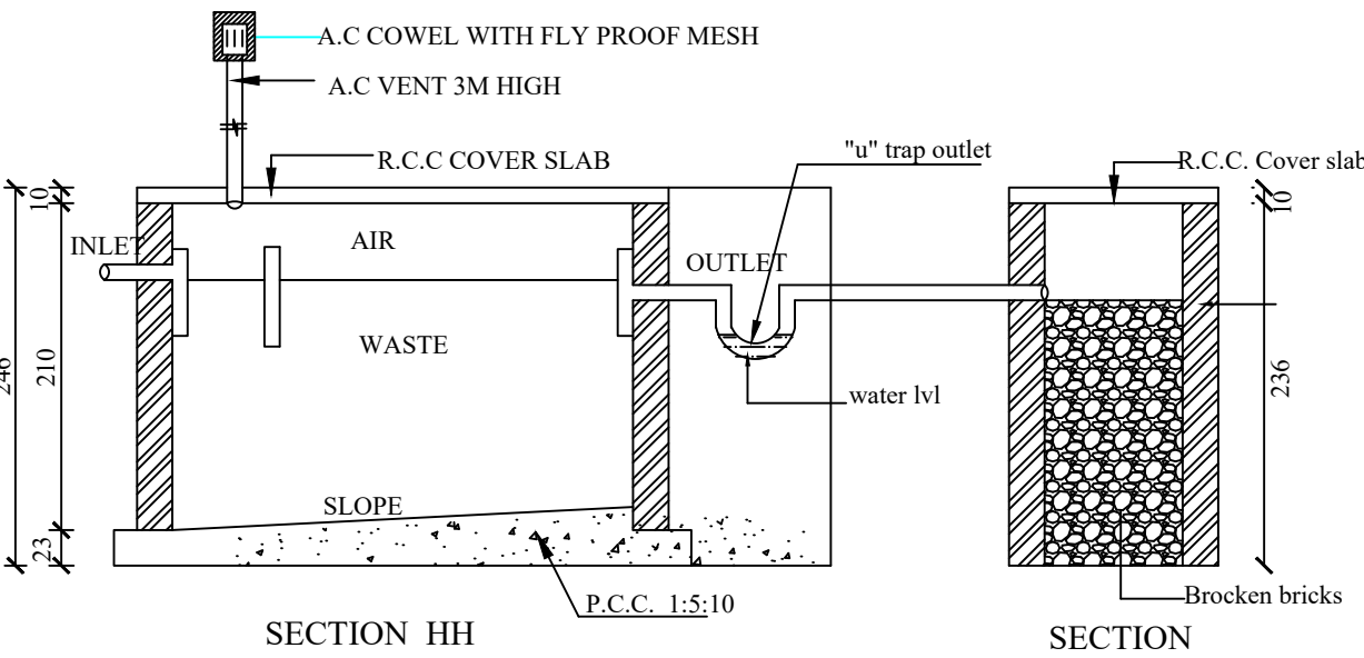
SECTION HH
