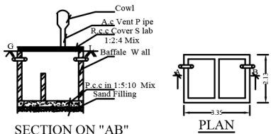
"SEPTIC TANK DETAILS"
