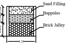
"RAINWATER TANK DETAILS"
