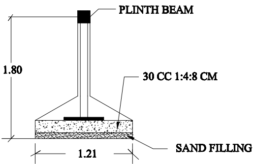
COLUMN DETAILS
