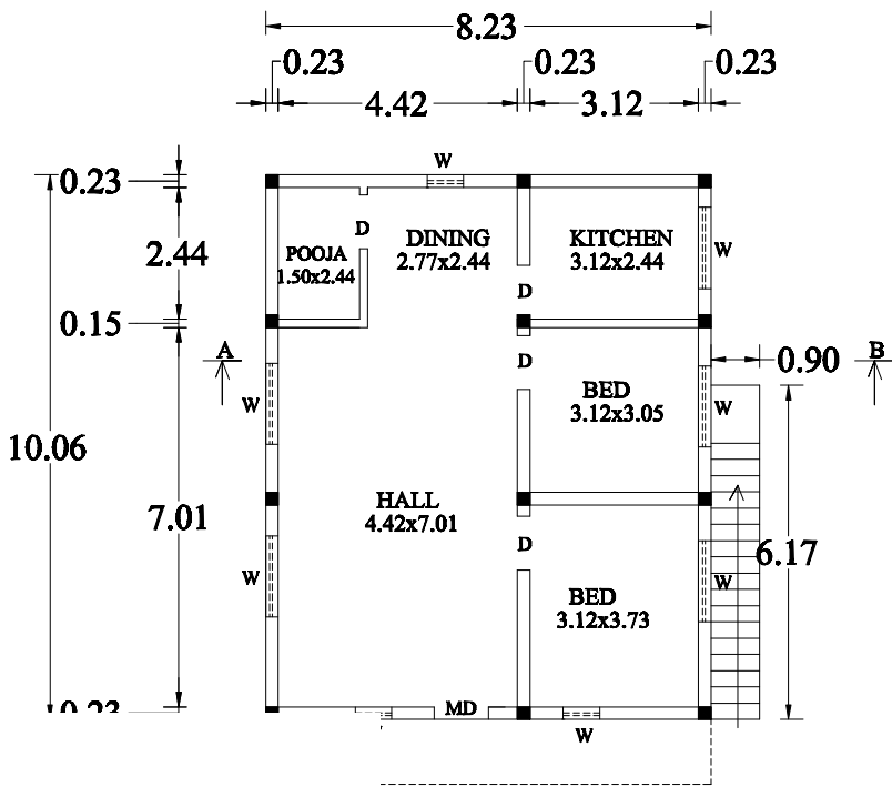
GROUND FLOOR WEST FACING
