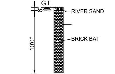
PERCULATION PIT
