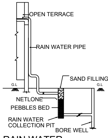
RAIN WATER
