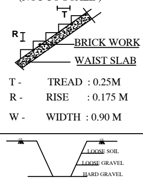
STAIRCASE DETAILS
