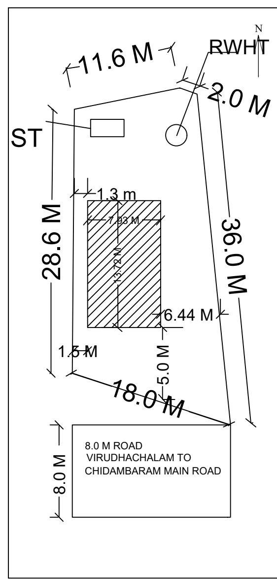
KEY PLAN
