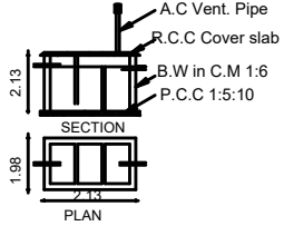
SEPTICTANK DETAILS
