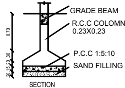
FOUNDATION DETAILS
