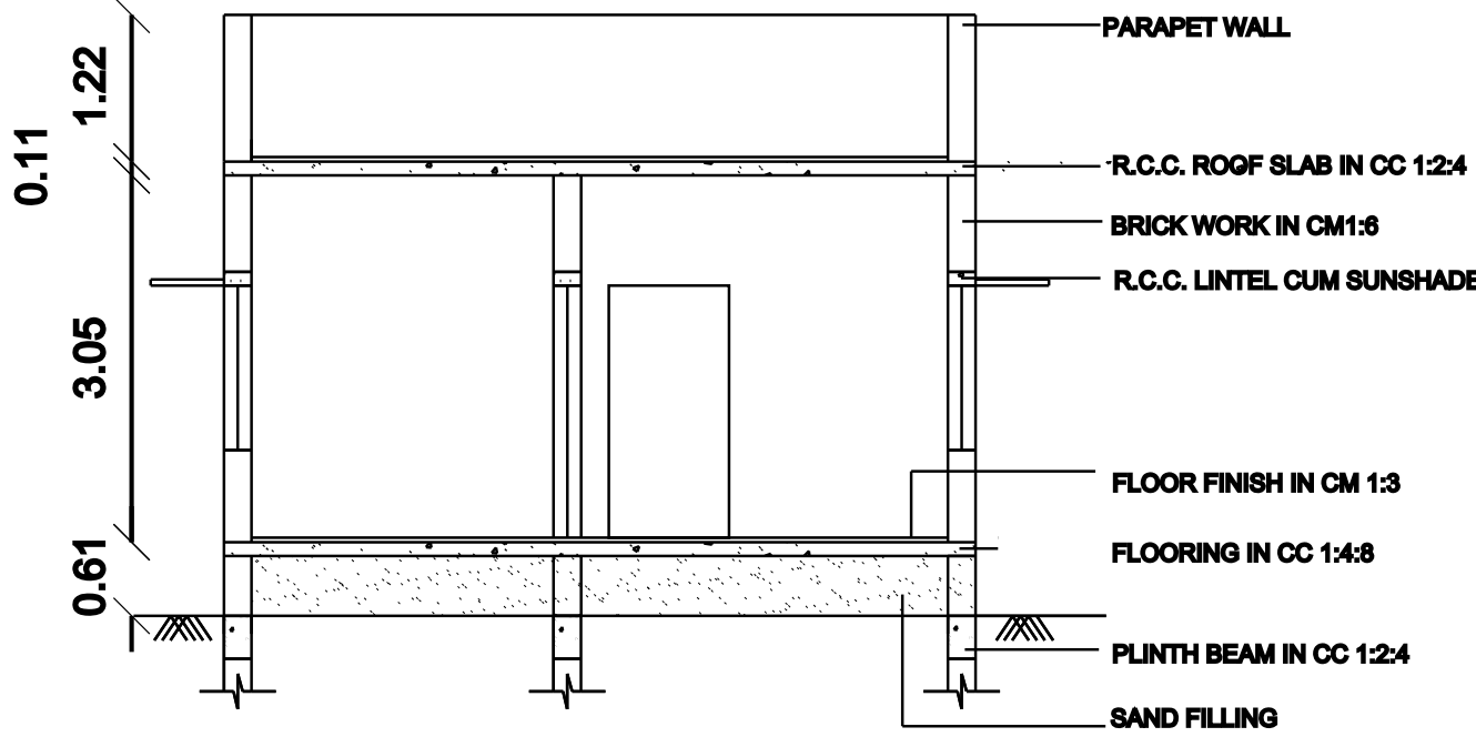
SECTION ON 'FB'
