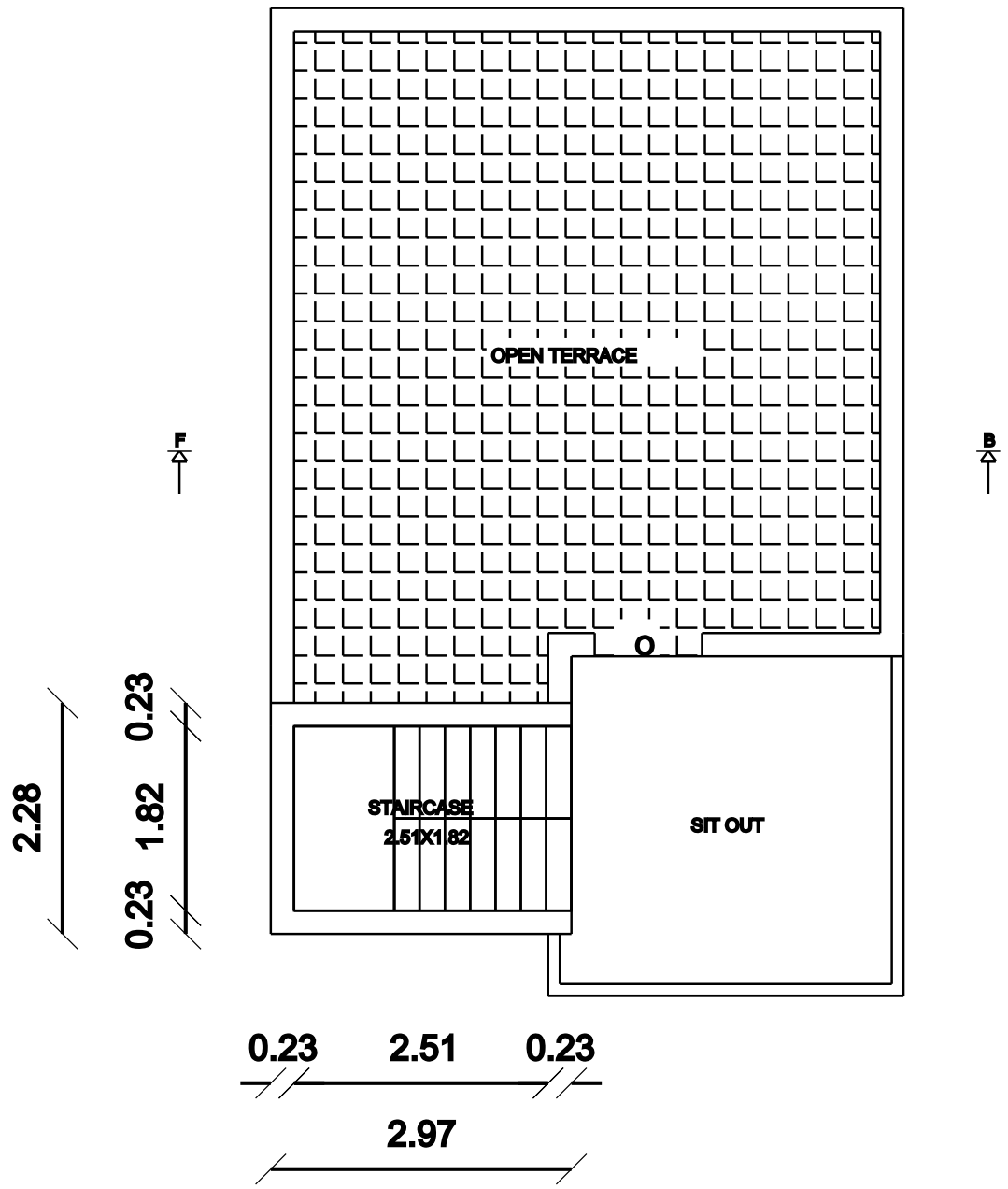
HEAD ROOM PLAN
