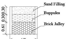
SECTION ON "AB"
