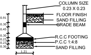
FOUNDATION DETAILS SCALE 1:500
