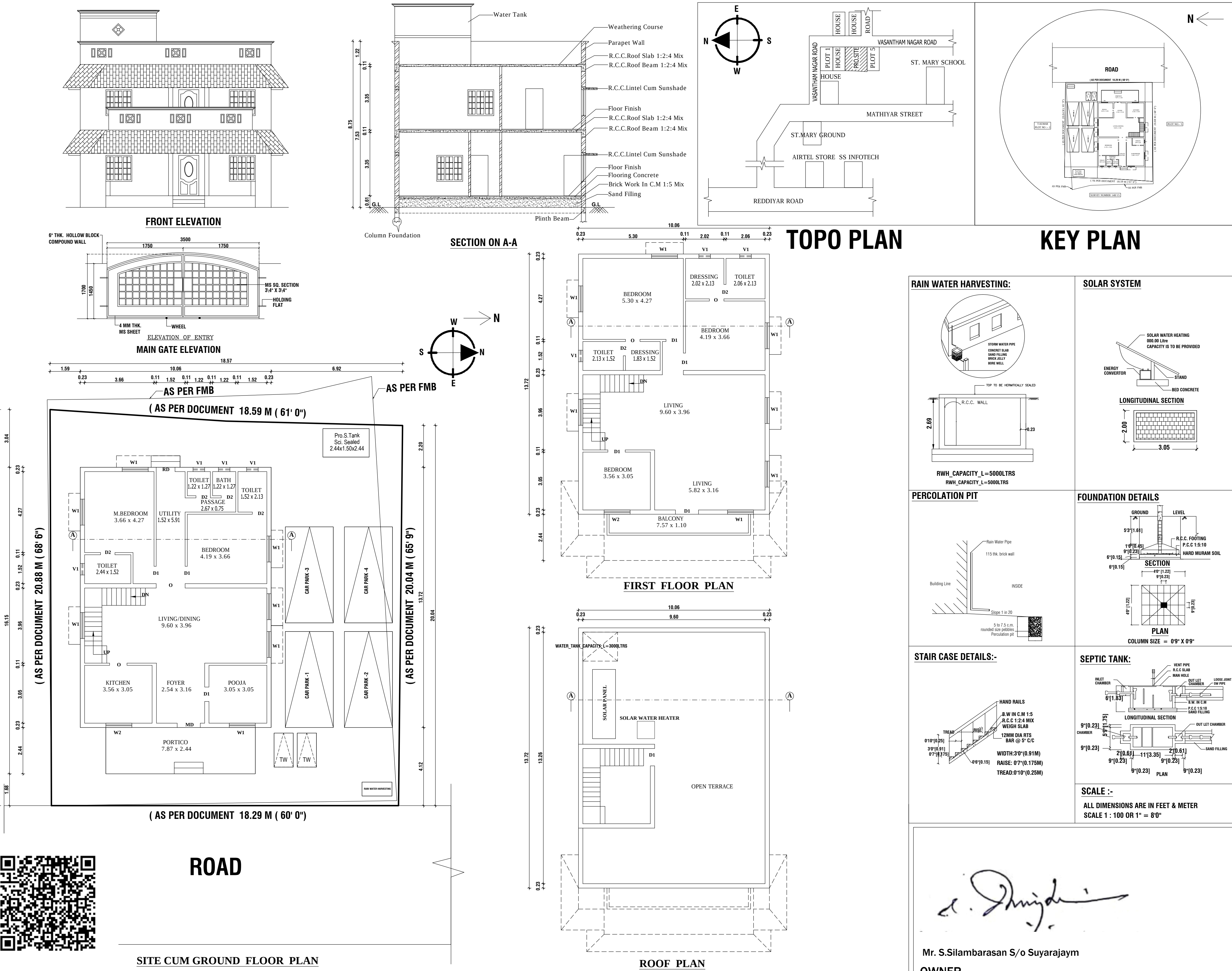
SITE CUM GROUND FLOOR PLAN
