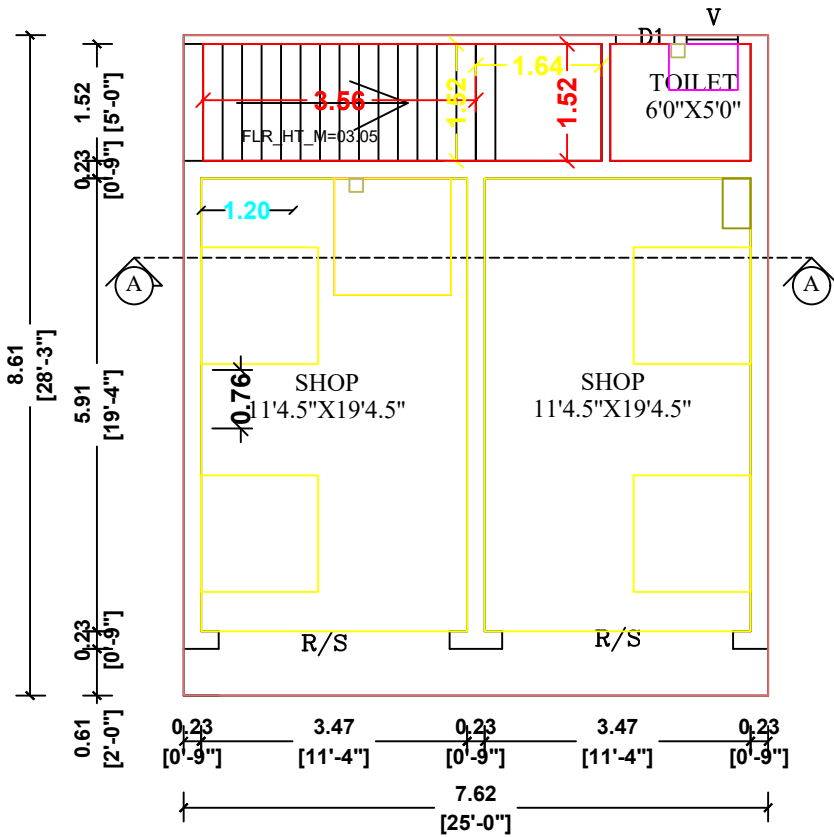
PROPOSED GROUND FLOOR PLAN (COMMERCIAL BUILDING)
