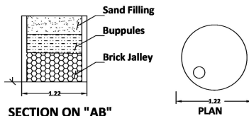
"RAINWATER TANK DETAILS"
