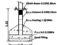
"FOUNDATION DETAILS"
