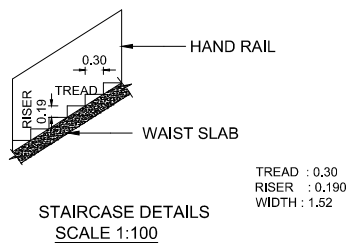
STAIRCASE DETAILS SCALE 1:100
