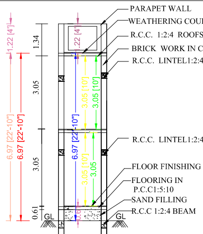
SECTION-AB
