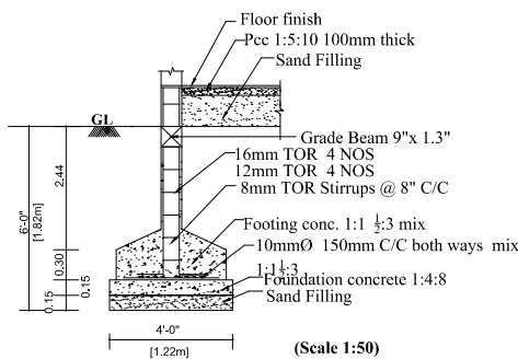
FOUNDATION DETAILS
