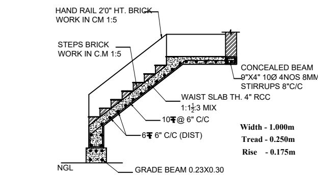
STAIRCASE DETAILS (Scale 1:50)
