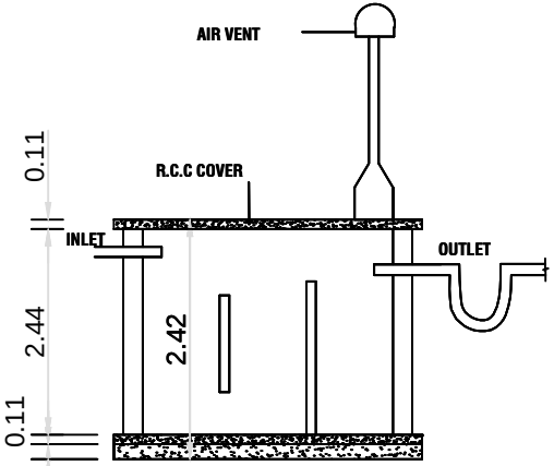
CROSS SECTION
