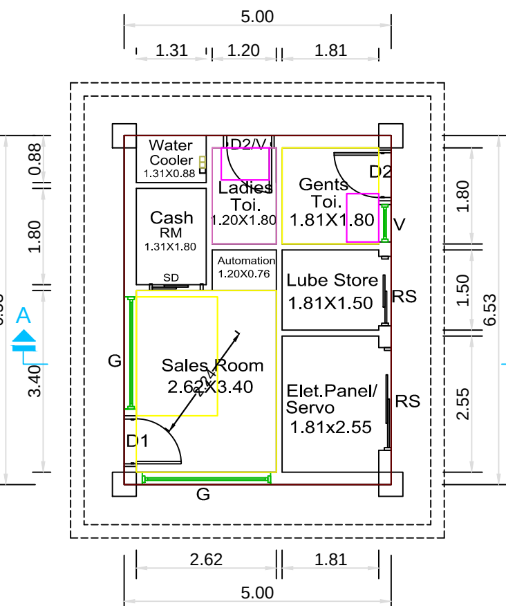
GROUND FLOOR PLAN ( OFFICE )
