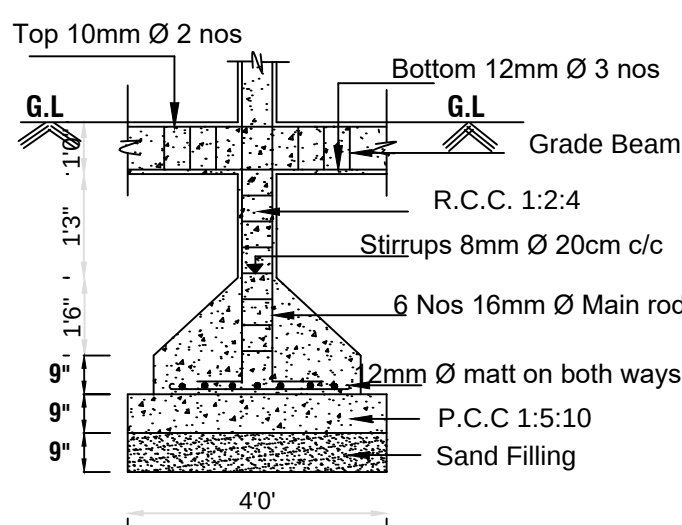
FOUNDATION DETAILS
