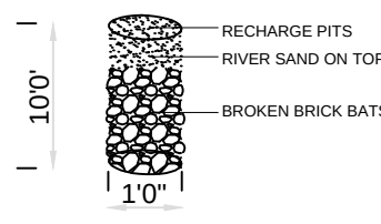
CONSTRUCTION DETAILS OF RECHARGE PITS
