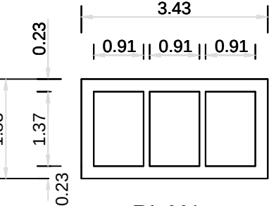
PLAN SEPTIC TANK DETAILS
