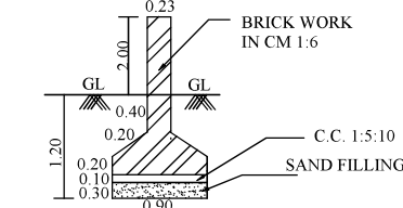
COMPOUND WALL SECTION
