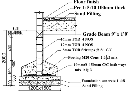
RCC COLUMN FOOTING
