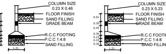
FOUNDATION DETAILS SCALE 1:500
