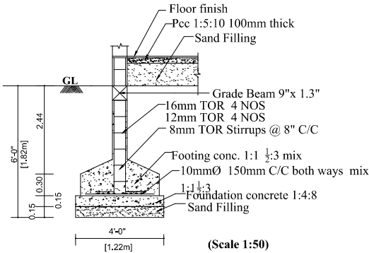
FOUNDATION DETAILS
