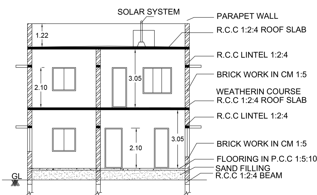
SECTION ON HH'
