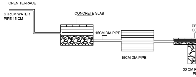
RAIN WATER HARVESTING SYSTEM NOT TO SCALE
