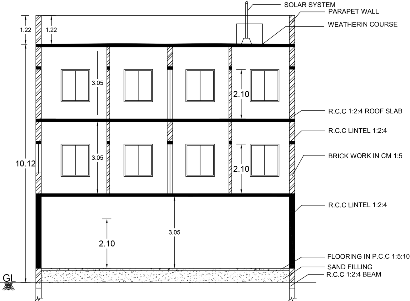
SECTION ON HH'
