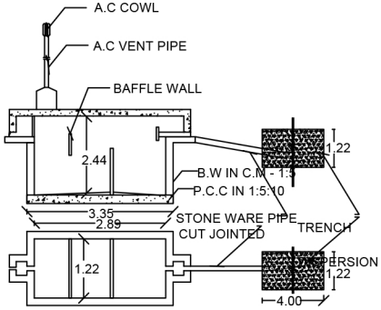
SEPTIC TANK DETAILS NOT TO SCALE
