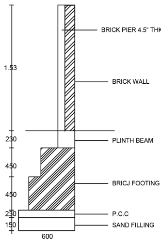
COMPOUND WALL DETAILS NOT TO SCALE
